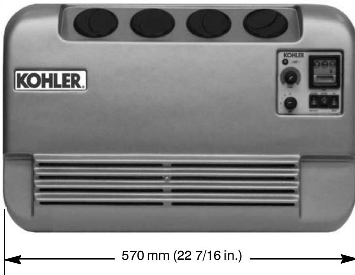
Evaporator Front-End View
